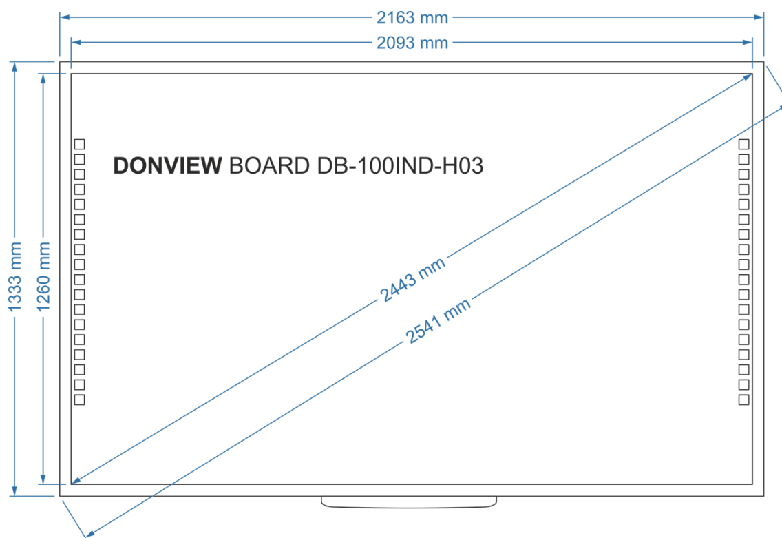
DONVIEW Board DB-100IND-H03
